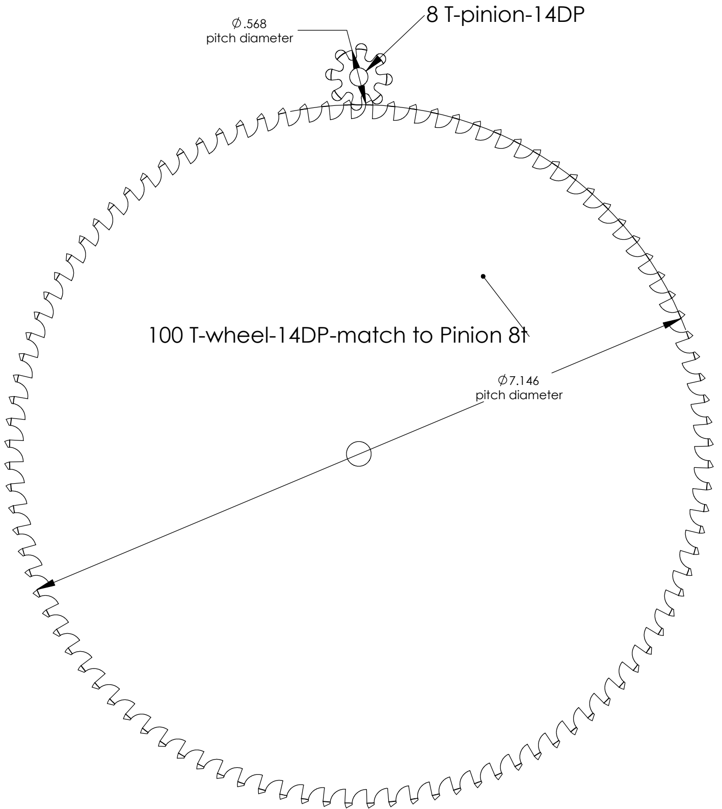
Full scale view of a large wheel and small pinion suitable for printing from A4 or 8.5x11 paper
